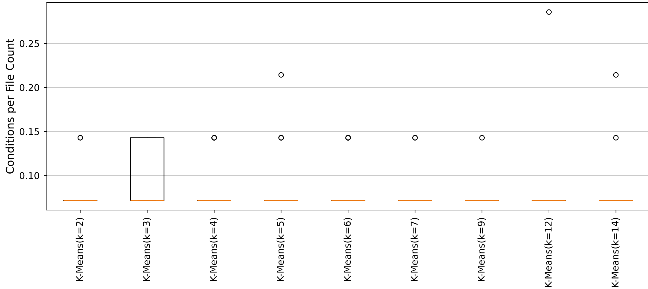
YARA Rules Conditions per File Count Distribution (Cluster7 Size14 dataset)
